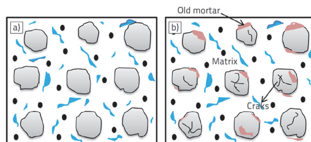
Figure 3. Schematic comparison of physical properties between: a) NCA; b) RCA [19]
