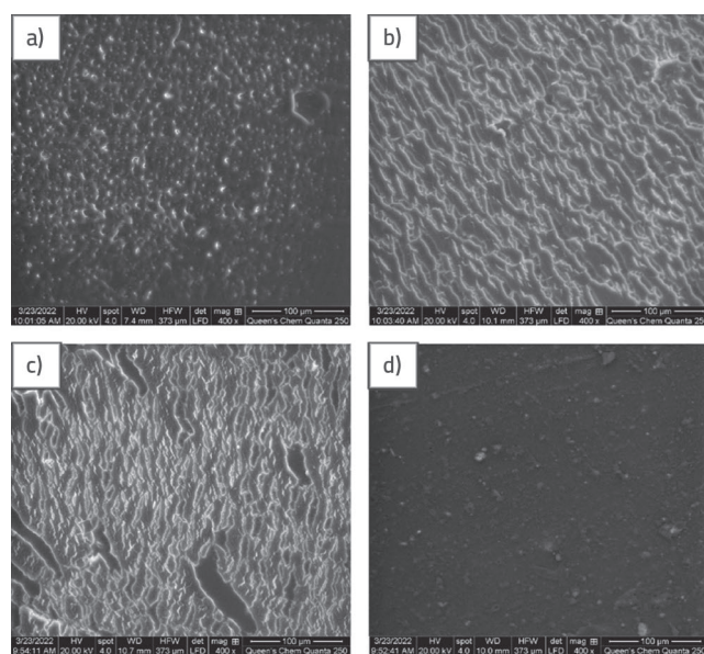
Figure 7. ESEM picture of the four plastic modified asphalts: a) 5 % PP; b) 5 % PS; c) 5 % HDPE; d) 5 % LDPE [61]
